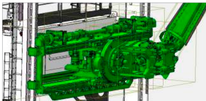
La parte mobile scorre verticalmente su guide cromate con cremagliera The mobile portal runs along two columns through chrome-plated guides with rack
